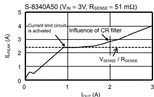
Figure 13 Measuring Coil Peak Current ( I_{\text{LPEAK}} )
