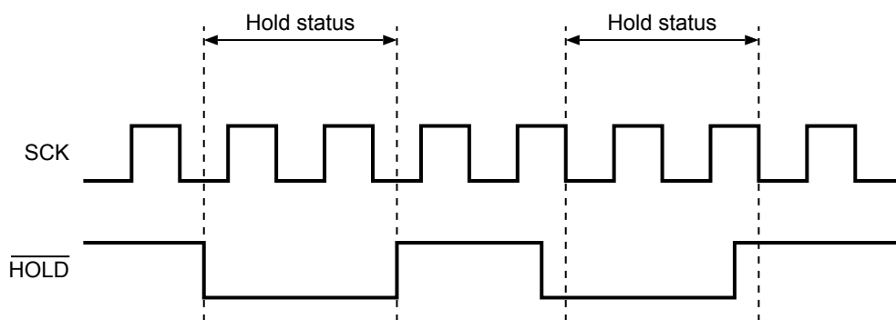
Figure 20 Hold Operation
