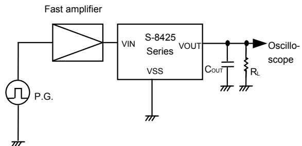
Figure 11 Test Circuit
