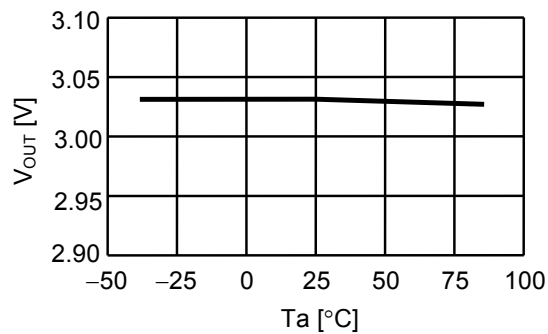
S-8730xxx Series
