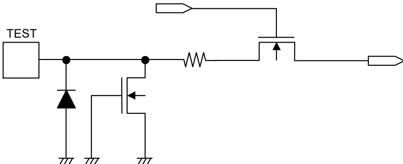
Figure 21 TEST Pin
