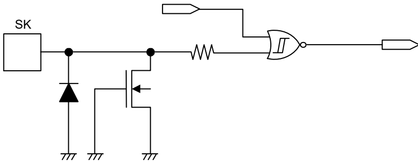
Figure 19 SK Pin
