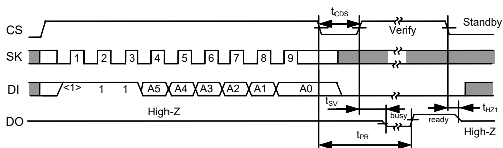
Figure 6 Data Erase Timing (S-93S46A)
