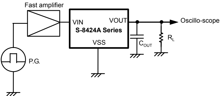
Figure 15 Test Circuit
