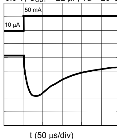
Figure 20 Ringing Waveform due to Load Variation (VOUT Pin)
