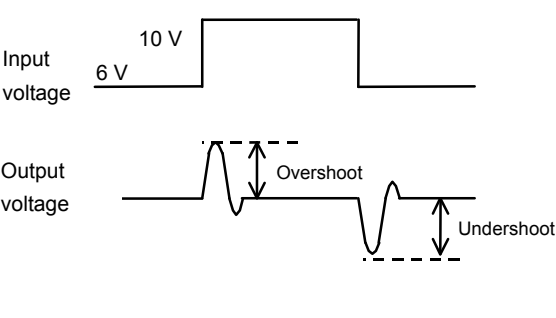
Figure 14 Power Supply Variation: 6 V and 10 V Square Waves
