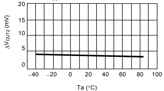
1.12 Load Stability ( V_{OUT} ) Temperature Characteristics
