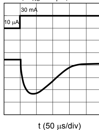
Figure 21 Ringing Waveform due to Load Variation (VRO Pin)
