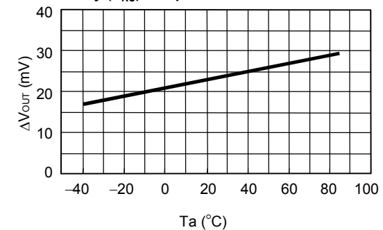
1.12 Load Stability ( V_{OUT} ) Temperature Characteristics
