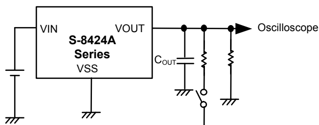
Figure 19 Test Circuit
