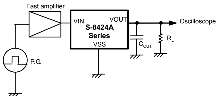
Figure 11 Test Circuit
