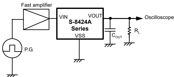
Figure 10 Test Circuit
