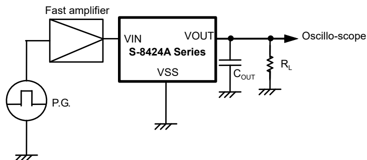
Figure 14 Test Circuit
