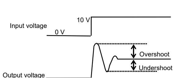
Figure 9 Power Supply Application: 0 V to 10 V Square Wave
