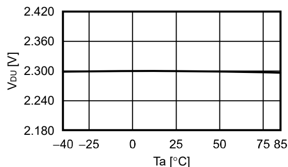
2.6 V_{DU} vs. T_a
