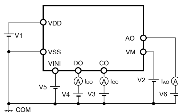
Figure 8 Test Circuit 4
