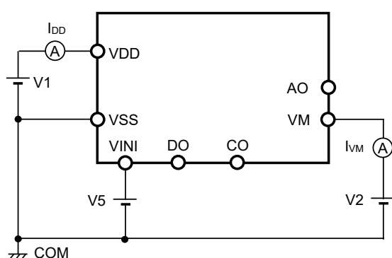
Figure 7 Test Circuit 3
