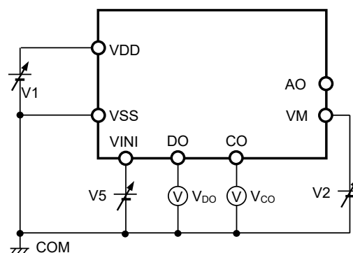
Figure 6 Test Circuit 2
