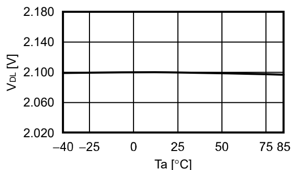
2.5 V_{DL} vs. T_a
