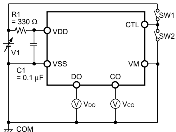
Figure 3 Test Circuit 1
