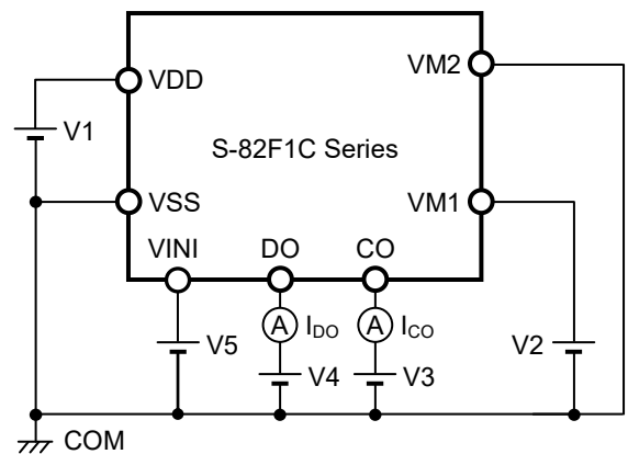
Figure 6 Test Circuit 4
