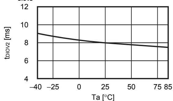
2. 15 t_{DIOV2} vs. T_a
