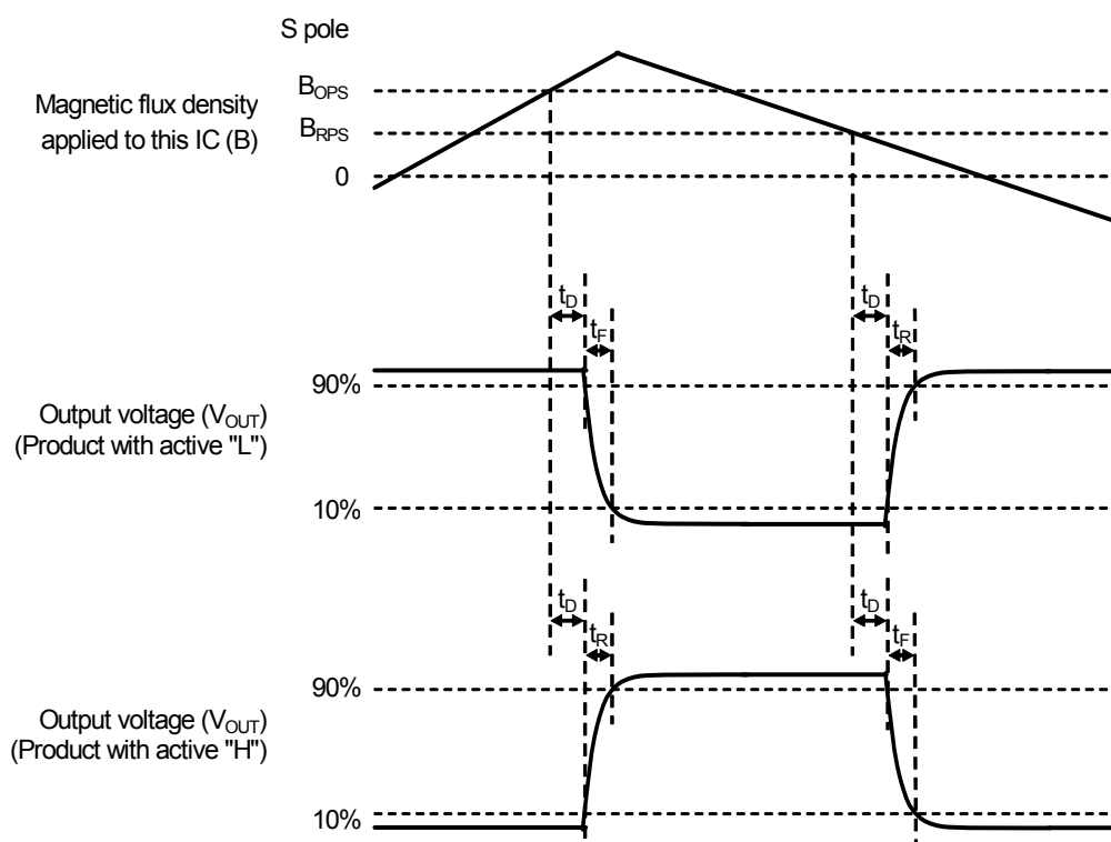
Figure 4 Operation Timing
