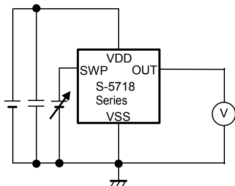
Figure 9 Test Circuit 7
