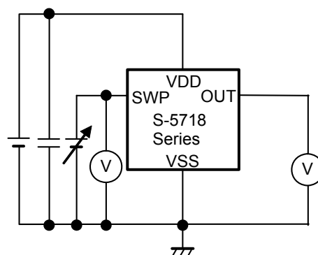
Figure 4 Test Circuit 2
