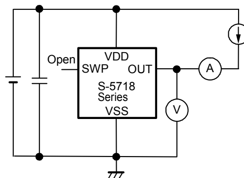
Figure 6 Test Circuit 4
