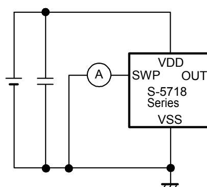
Figure 8 Test Circuit 6
