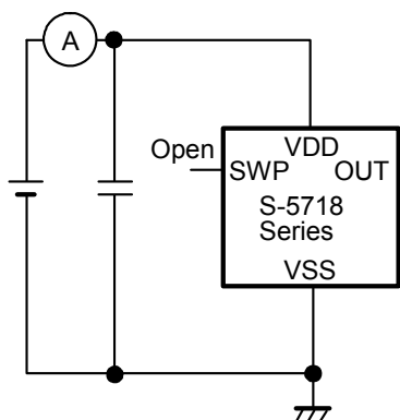
Figure 3 Test Circuit 1
