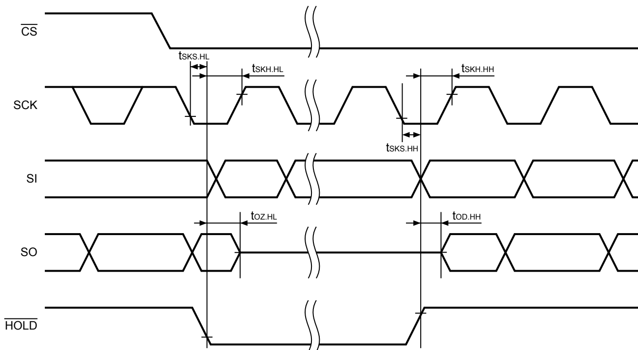
Figure 4 Hold Timing
