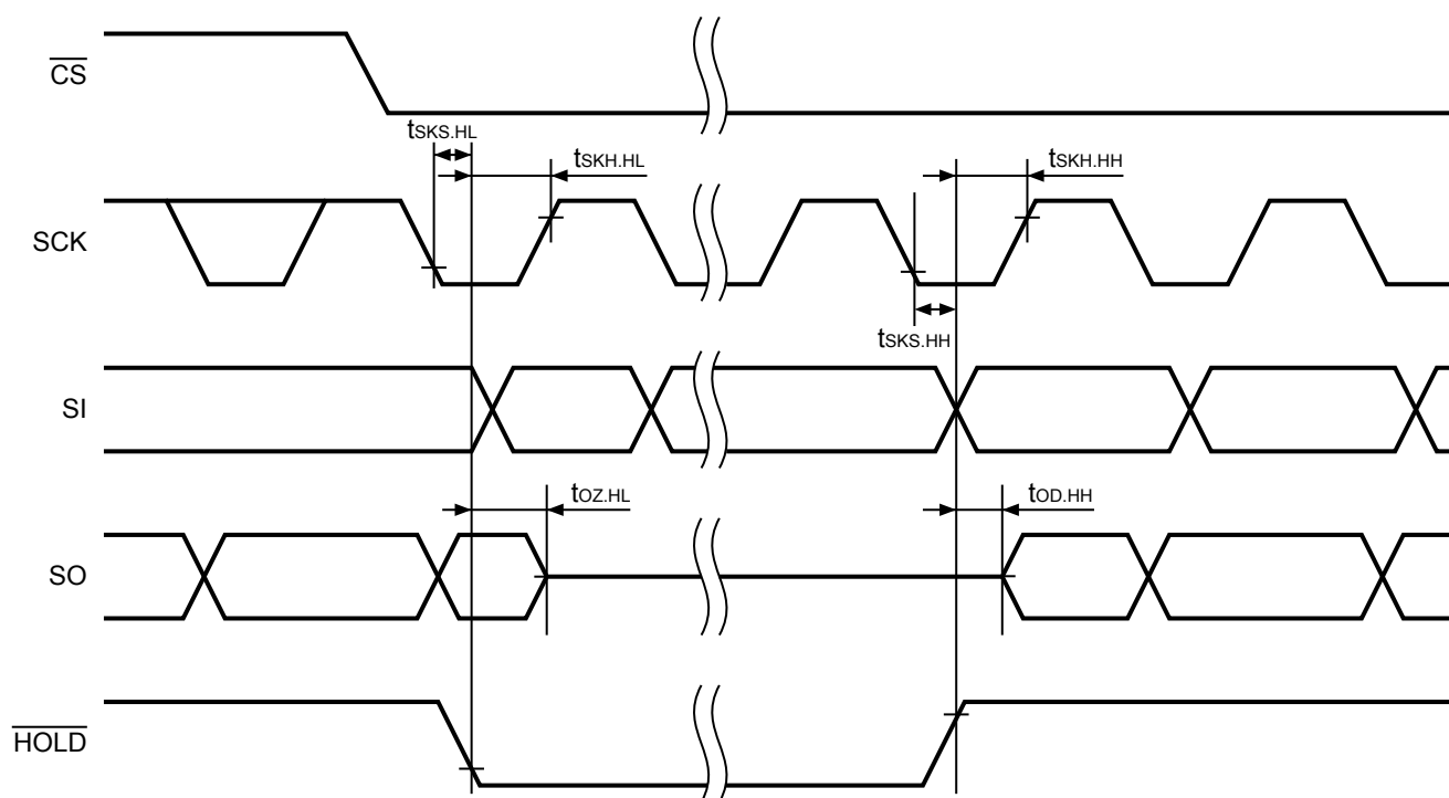
Figure 5 Hold Timing
