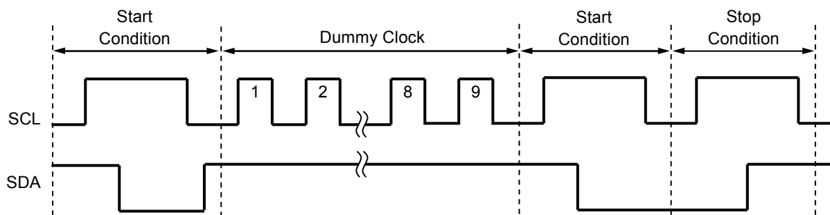
Figure 24 Resetting S-24C256C
