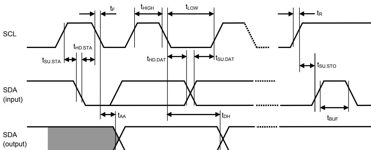
Figure 6 Bus Timing
