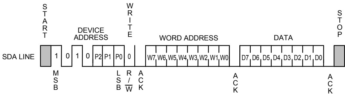
Figure 13 Byte Write
