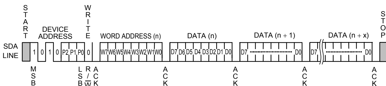
Figure 14 Page Write
