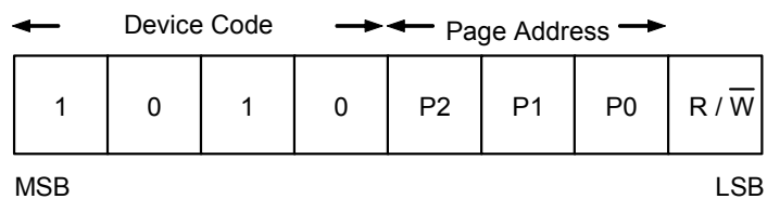
Figure 12 Device Address
