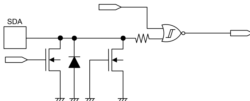
Figure 22 SDA Pin
