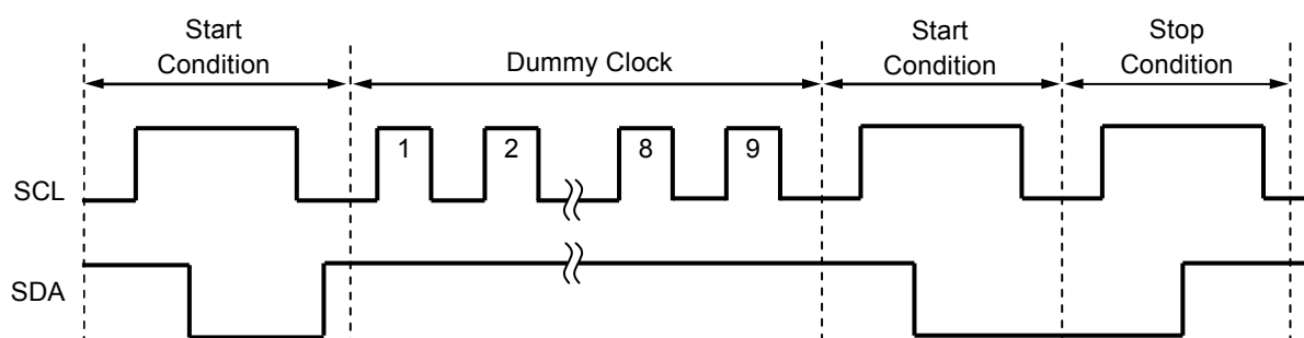
Figure 25 Resetting S-24C08C
