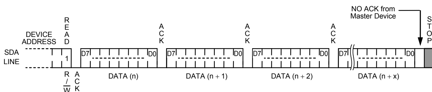
Figure 19 Sequential Read
