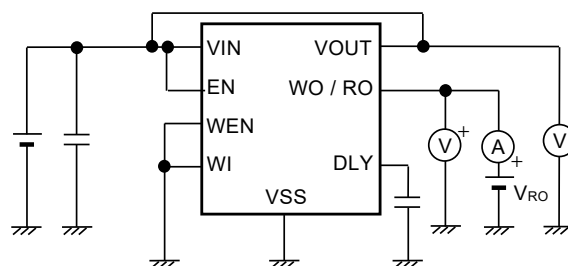
Figure 14 Test Circuit 6
