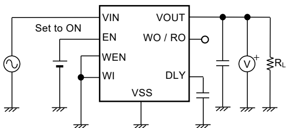
Figure 11 Test Circuit 3
