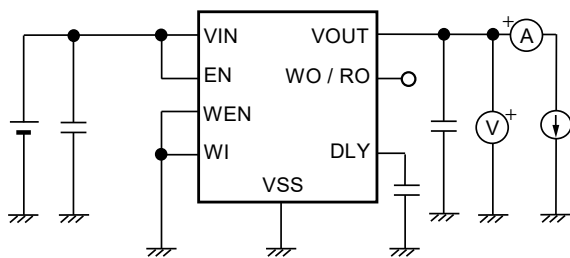
Figure 9 Test Circuit 1
