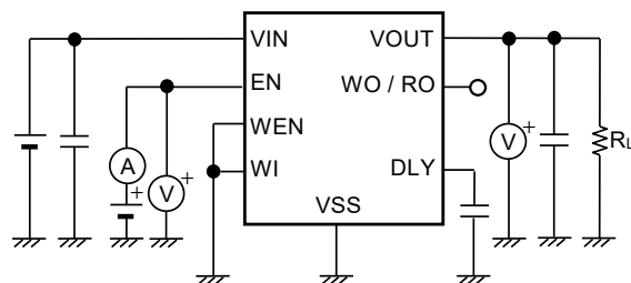
Figure 12 Test Circuit 4
