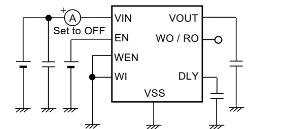
Figure 18 Test Circuit 10
