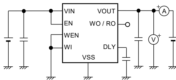
Figure 10 Test Circuit 2
