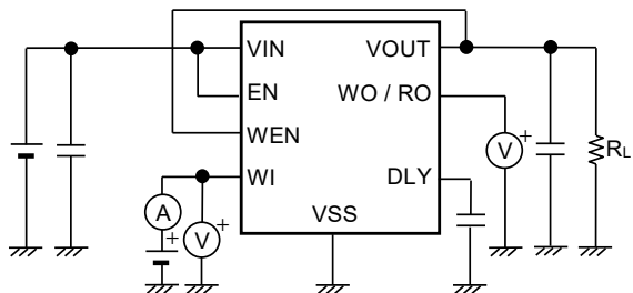
Figure 15 Test Circuit 7
