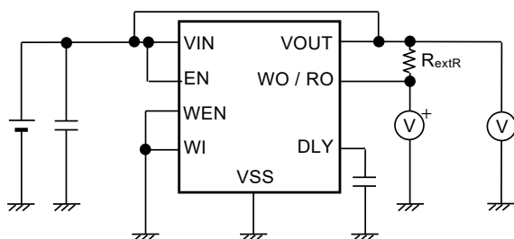
Figure 13 Test Circuit 5
