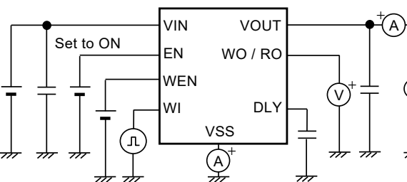
Figure 17 Test Circuit 9
