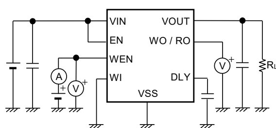
Figure 16 Test Circuit 8
