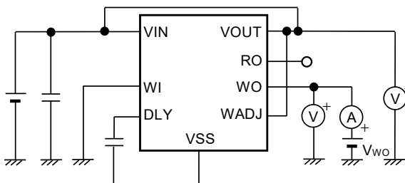
Figure 30 Test Circuit 9
