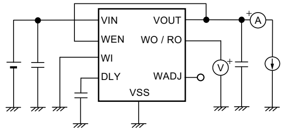
Figure 17 Test Circuit 6
