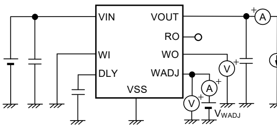
Figure 28 Test Circuit 7
