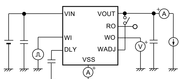
Figure 31 Test Circuit 10
