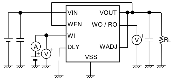
Figure 19 Test Circuit 8
