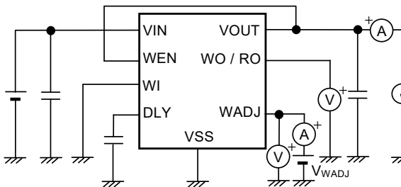
Figure 18 Test Circuit 7
