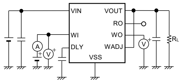
Figure 29 Test Circuit 8
