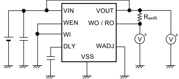
Figure 15 Test Circuit 4
