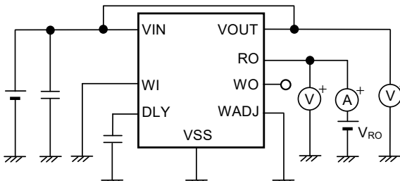
Figure 26 Test Circuit 5
