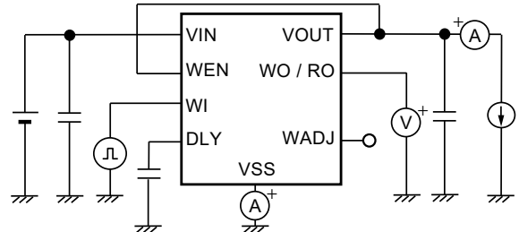
Figure 21 Test Circuit 10
