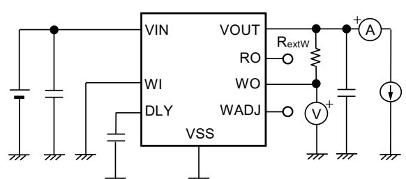
Figure 27 Test Circuit 6
