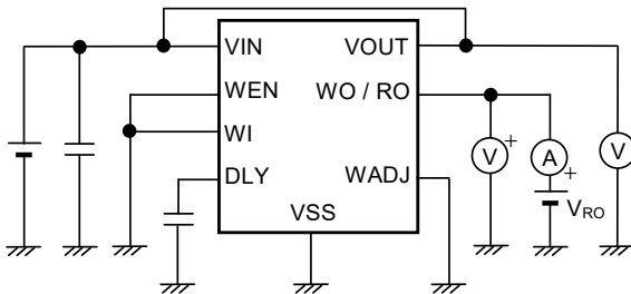
Figure 16 Test Circuit 5
