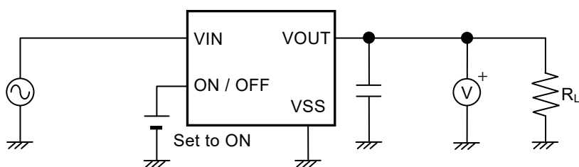
Figure 12 Test Circuit 5
