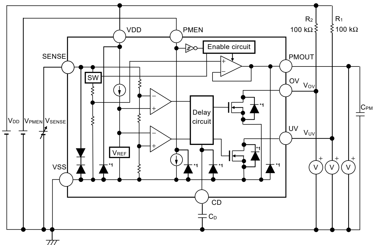
Figure 19 Operation of S-191L/191N Series L / P type
