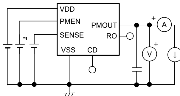
Figure 8 Test Circuit 4
