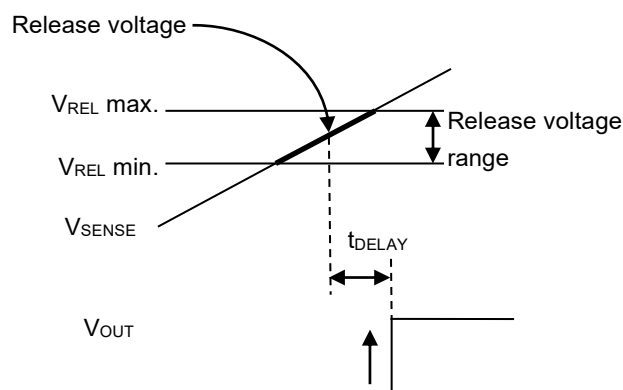
Figure 11 Release Voltage
