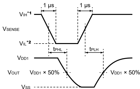
Figure 21 Test Condition of Response Time
