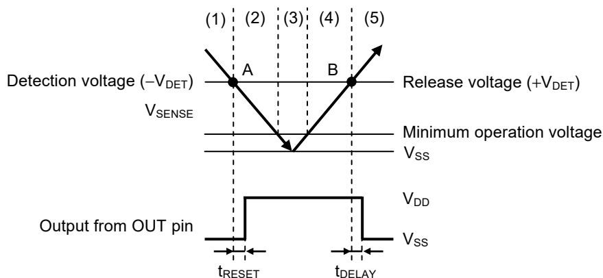
Figure 38 Operation of S-19110 Series R Type
