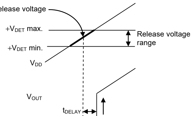
Figure 19 Release Voltage (VDD Detection Product)
