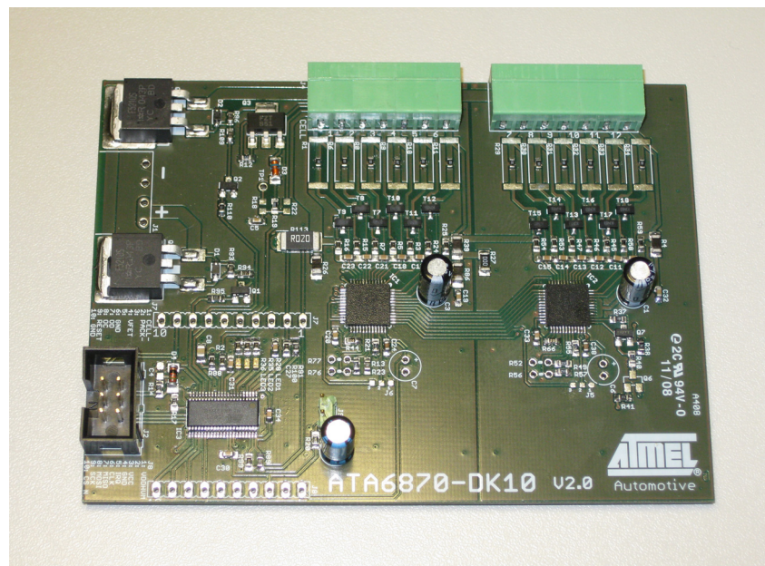
Figure 1. Atmel ATA6870-DK10
