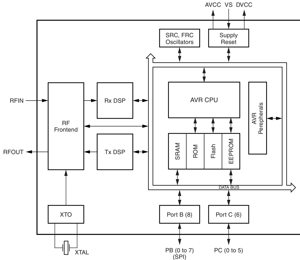
Figure 1-6. Circuit Overview
