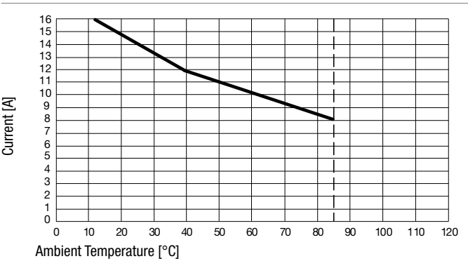
Variants 2 0751.0110 and 0751.0231
