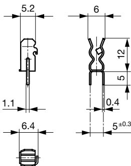
Variants 0751.0052 and 0751.0062
