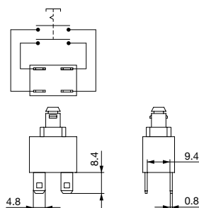
Contact Layout double-pole
