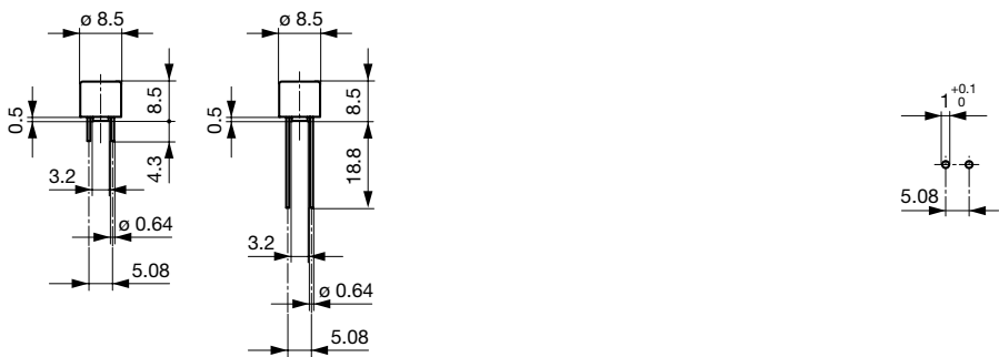
Drilling diagram
