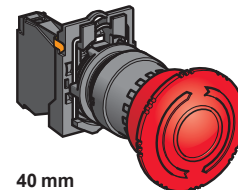
Turn to release (EN/ISO 13850: 2006) XB5AS8●4 see page 110
