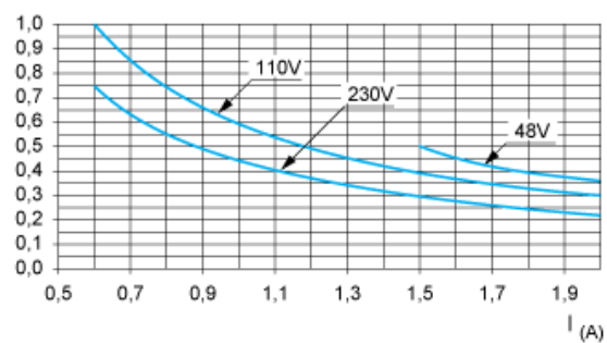
AC15 curves
