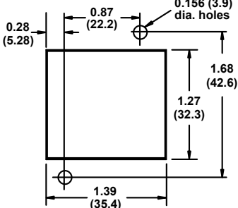
Chassis Cutout
