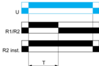
2 timed outputs (R1/R2) or 1 timed output (R1) and 1 instantaneous output (R2 inst.)
