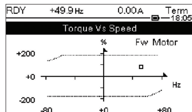
Torque Vs Speed display
