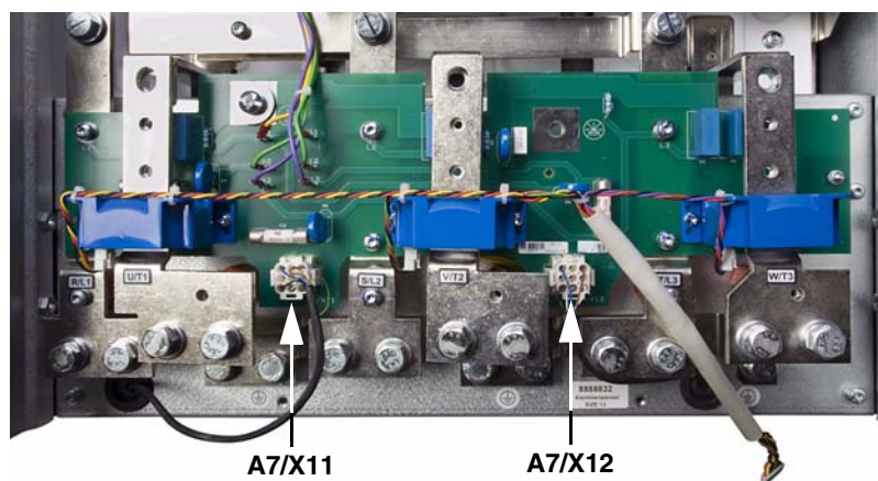
Figure 32: Filter Board Fan Connections
