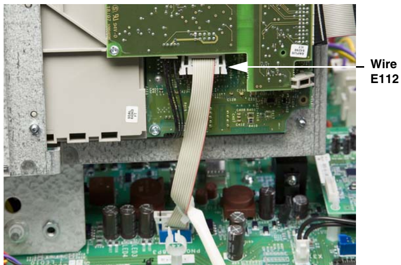
Figure 107: Control Module Assembly Back
