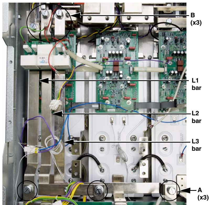
Figure 57: L1, L2, L3 Bus Bars
