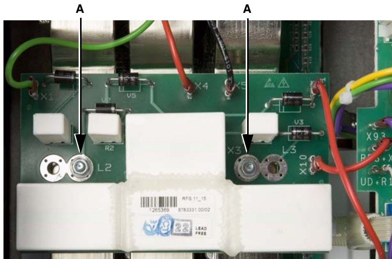
Figure 14: SCR Snubber Board
