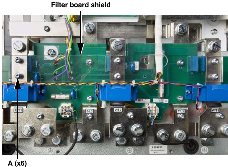
Figure 37: Filter Board Shield
