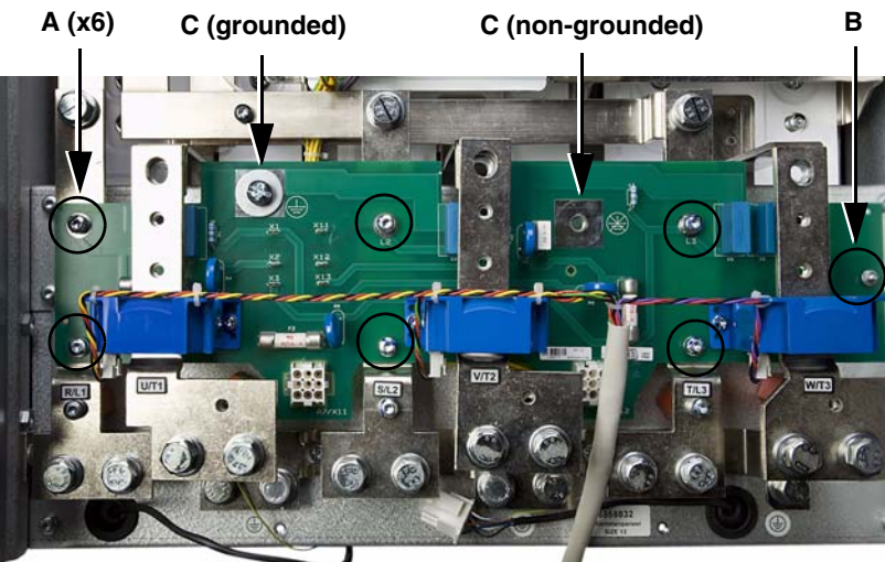
Figure 30: Filter Board Mounting Hardware
