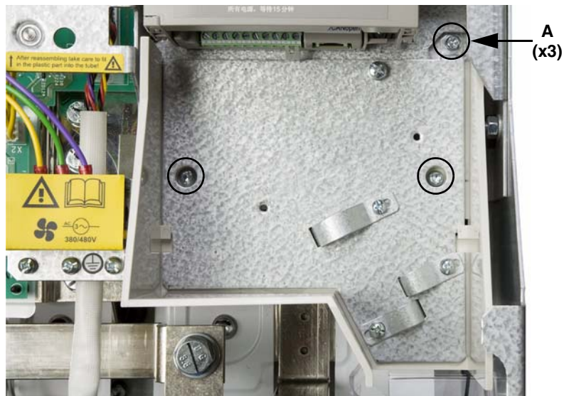
Figure 18: EMC Tray
