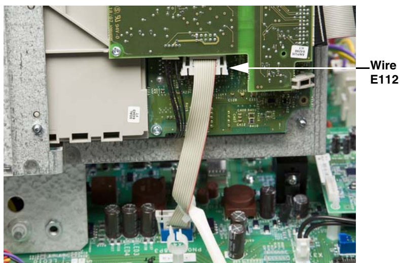
Figure 47: Control Module Assembly Back
