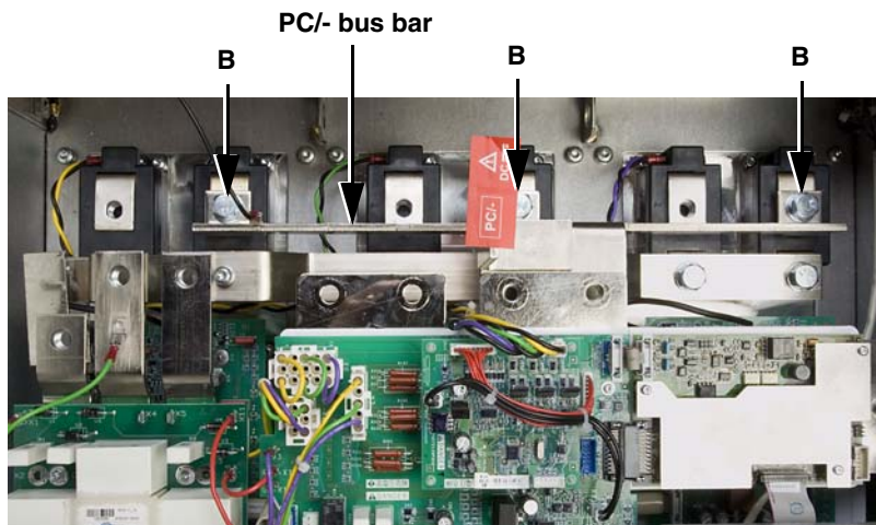
Figure 79: PC/- Bus Bar
