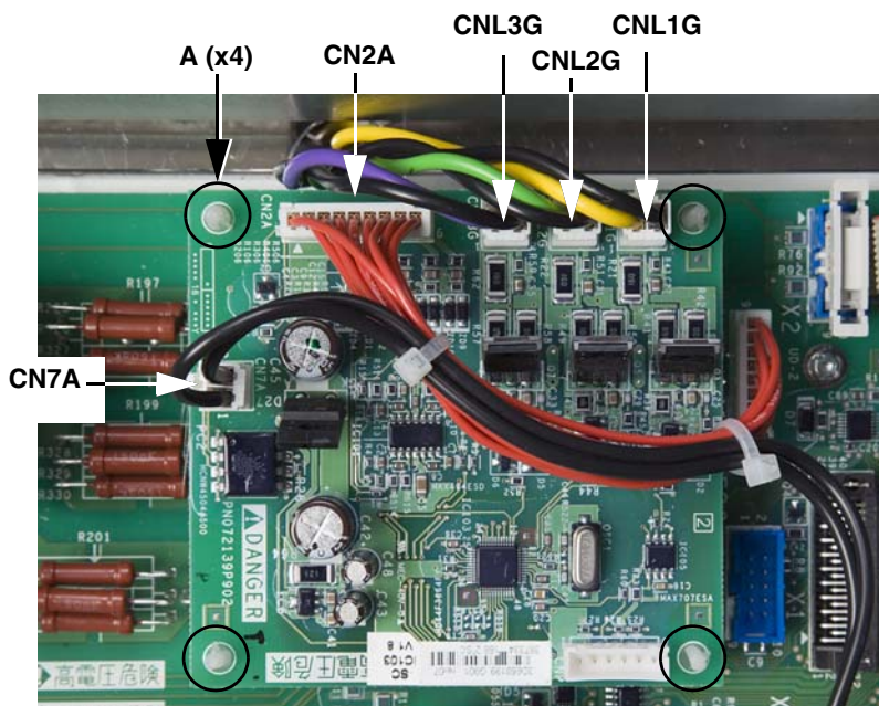
Figure 12: Soft Charge Board
