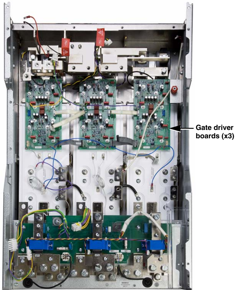
Figure 4: Gate Driver Boards
