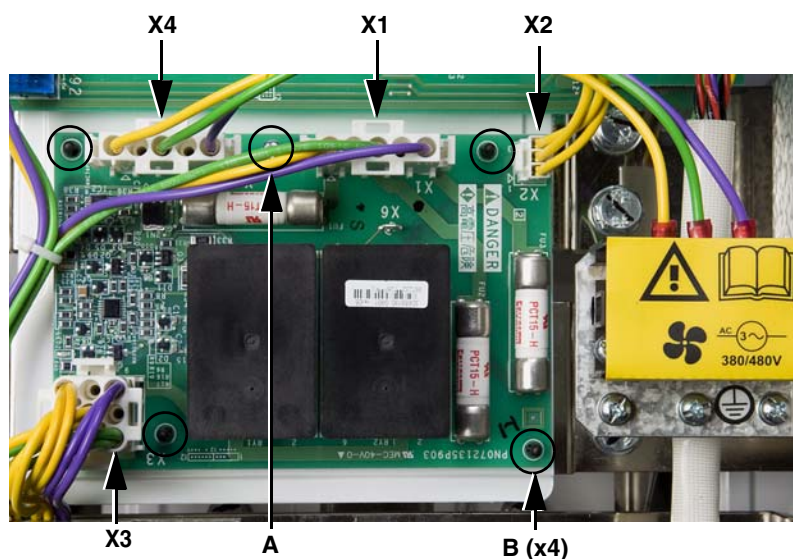
Figure 15: Fan Control Board
