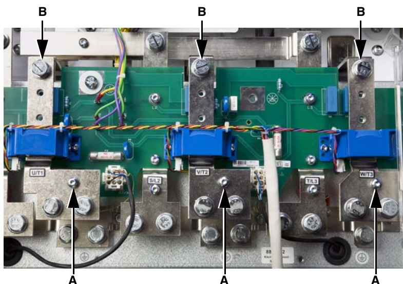
Figure 35: Output Bus Bars
