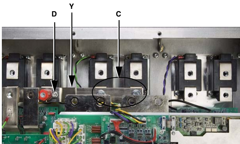
Figure 86: SCR Buswork, Phase V
