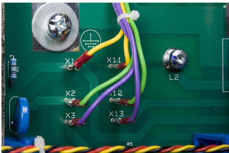
Figure 24: Filter Board Connections
