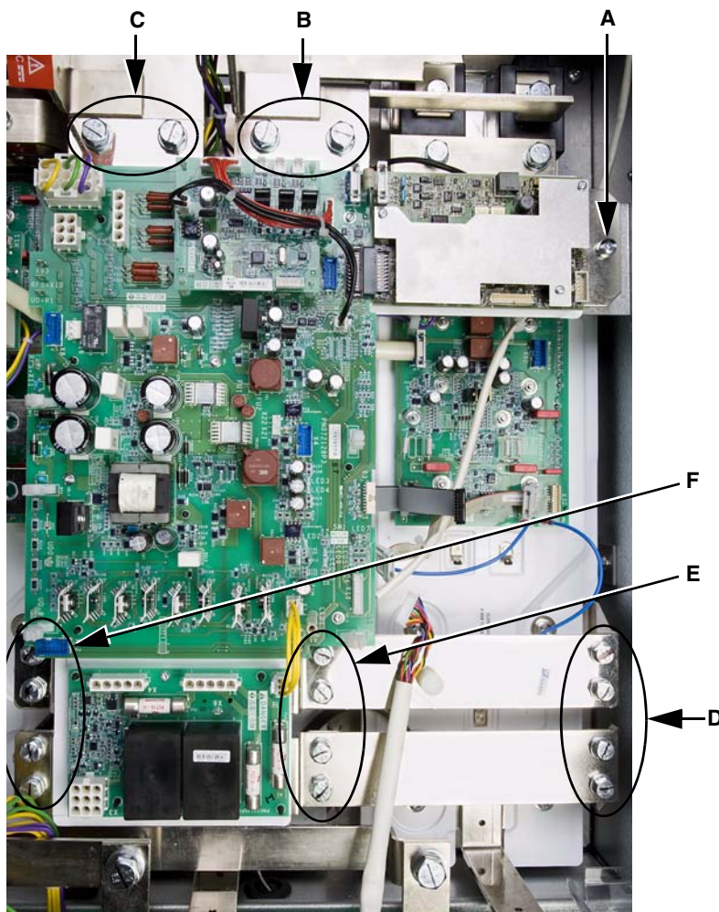
Figure 99: Bus Plate Assembly
