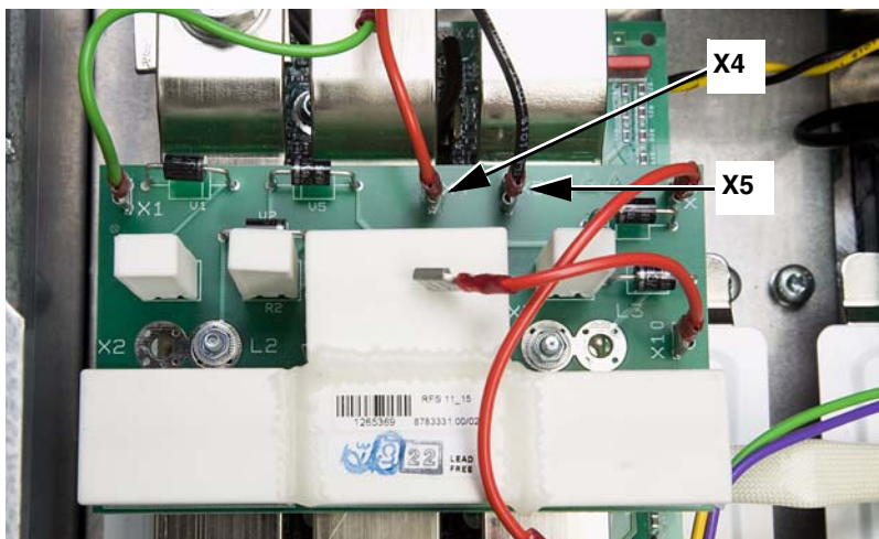
Figure 57: L1, L2, L3 Bus Bars
