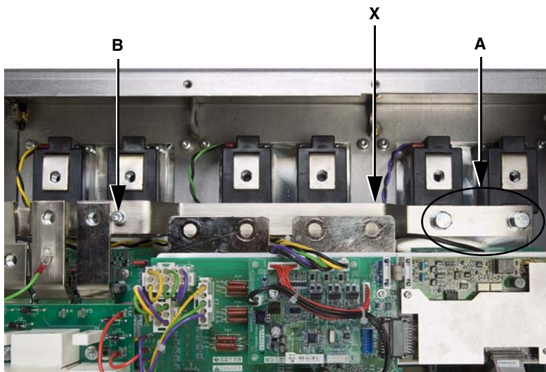
Figure 87: SCR Buswork, Phase W
