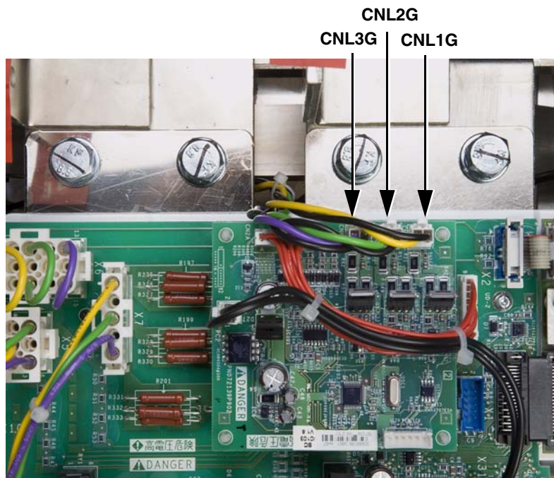
Figure 53: Soft Charge Board Connections
