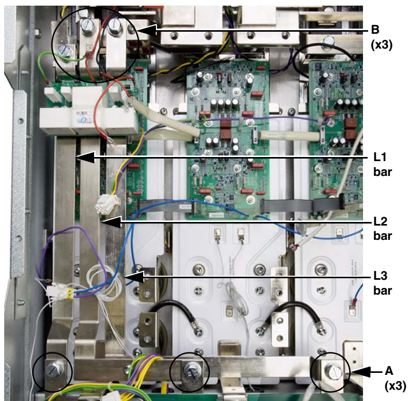
Figure 98: SCR Snubber Board
