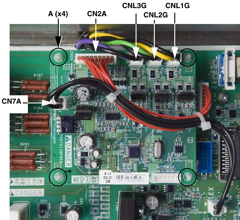
Figure 60: Soft Charge Board
