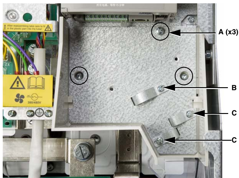
Figure 10: EMC Tray
