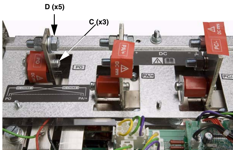
Figure 93: Fan Plate with Bus Bar Detail
