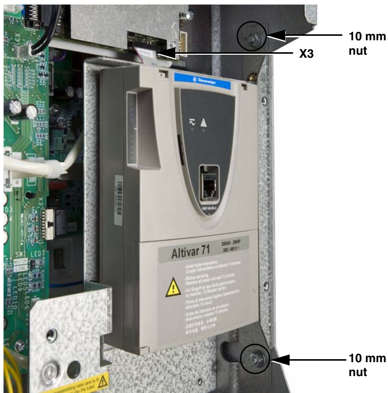
Figure 108: Control Module Assembly Front
