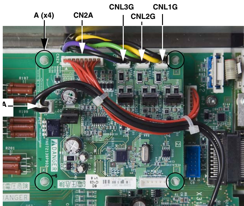
Figure 63: Soft Charge Board
