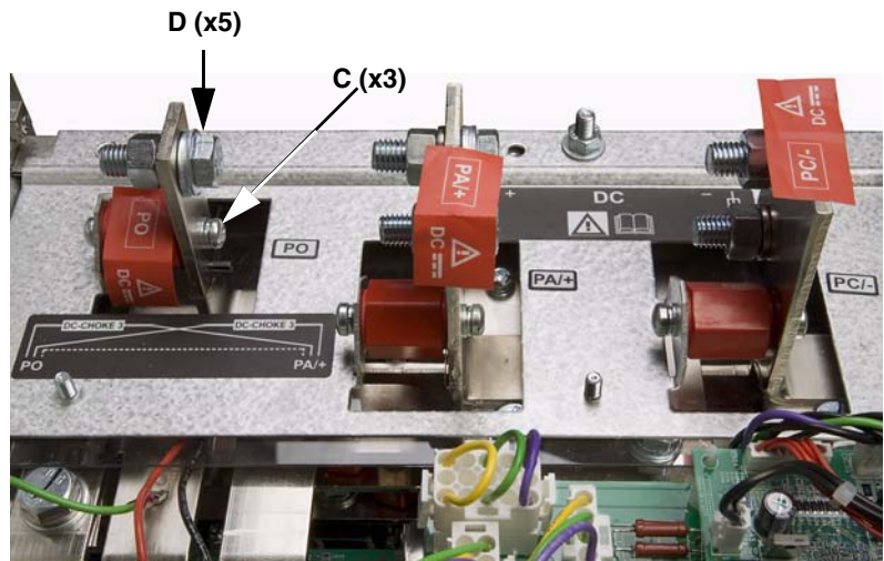
Figure 105: Fan Plate with Bus Bar Detail
