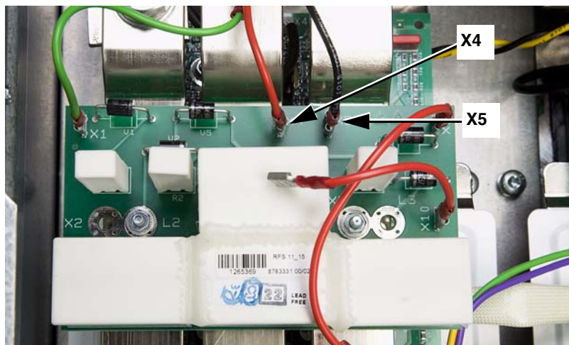
Figure 98: SCR Snubber Board
