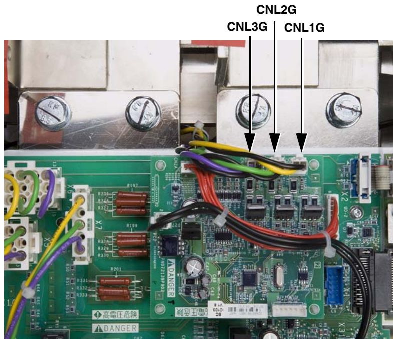
Figure 101: Soft Charge Board Connections
