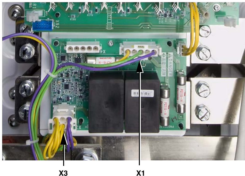
Figure 54: Fan Control Board Connections X1 and X3
