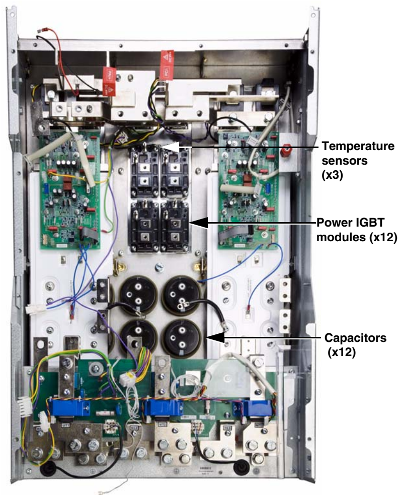
Figure 5: Temperature Sensors, Power IGBT Modules, and Capacitors
