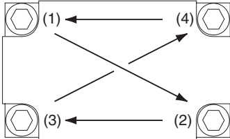
Figure 83: Torque Sequence
