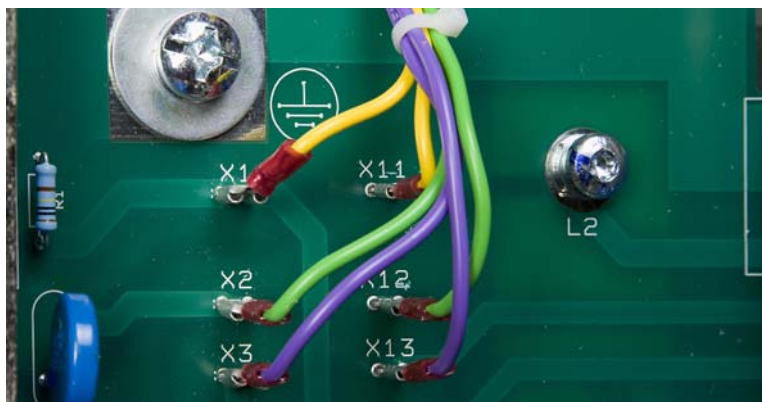
Figure 33: Filter Board Connections
