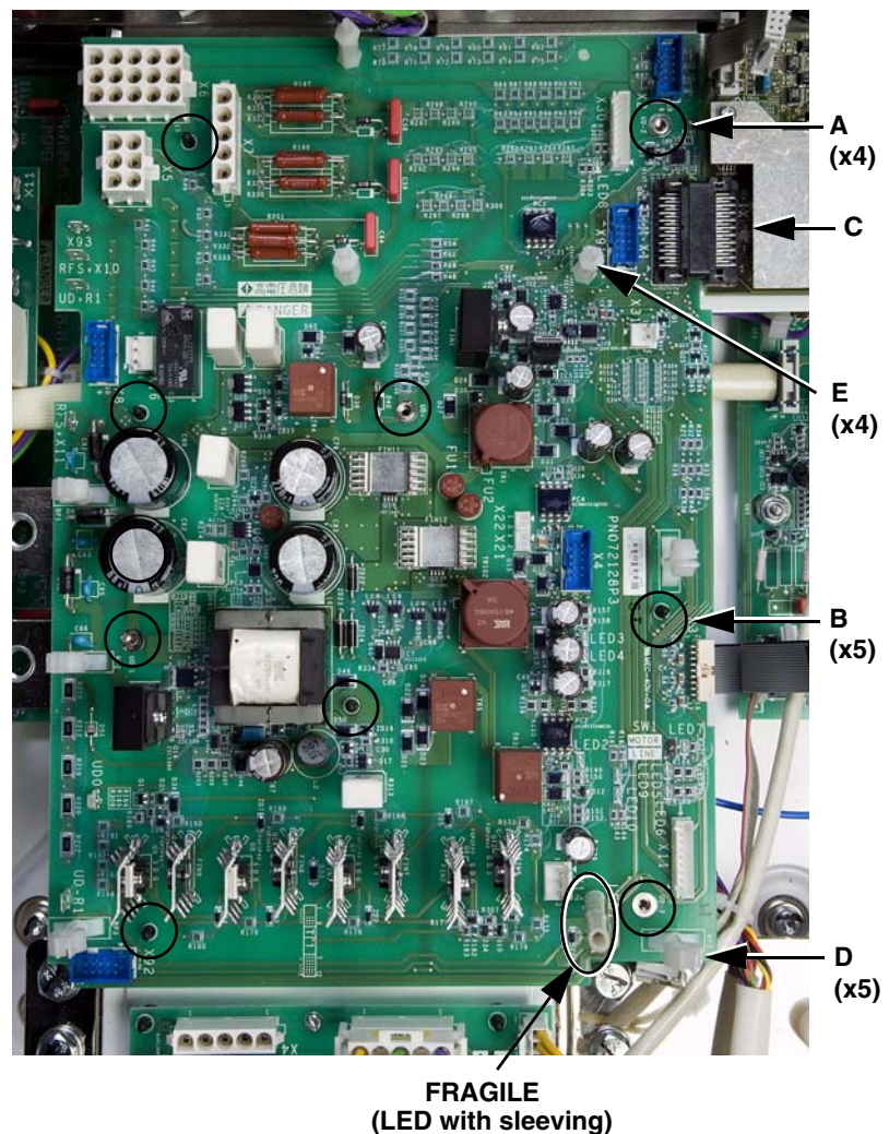
Figure 62: Power Board
