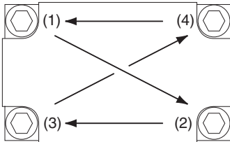
Figure 70: Torque Sequence
