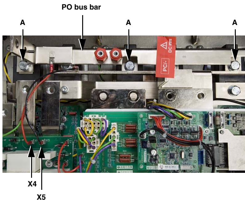
Figure 78: PO Bus Bar
