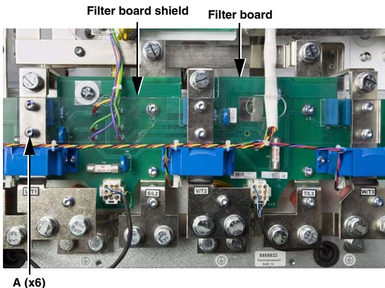
Figure 19: Filter Board Shield
