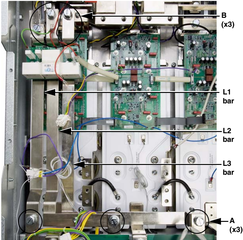
Figure 68: SCR Snubber Board
