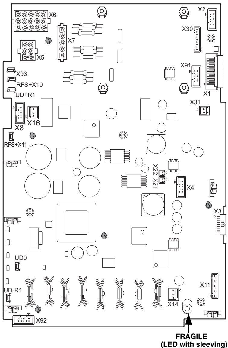
Figure 61: Power Board Connections
