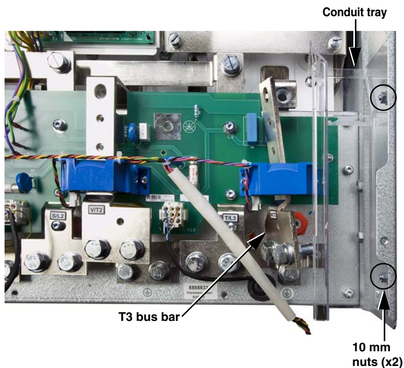
Figure 23: Conduit Tray
