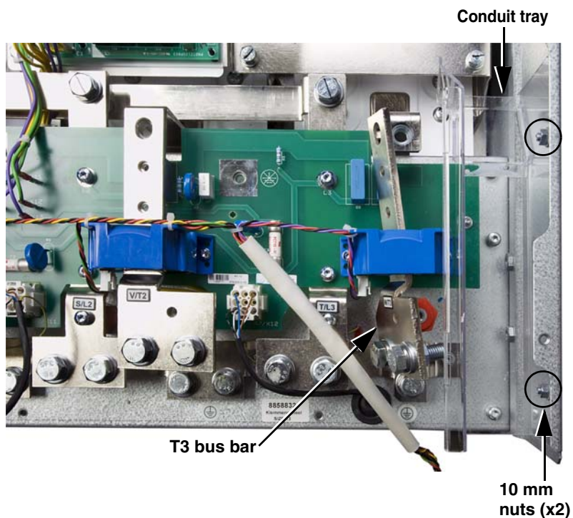
Figure 34: Conduit Tray
