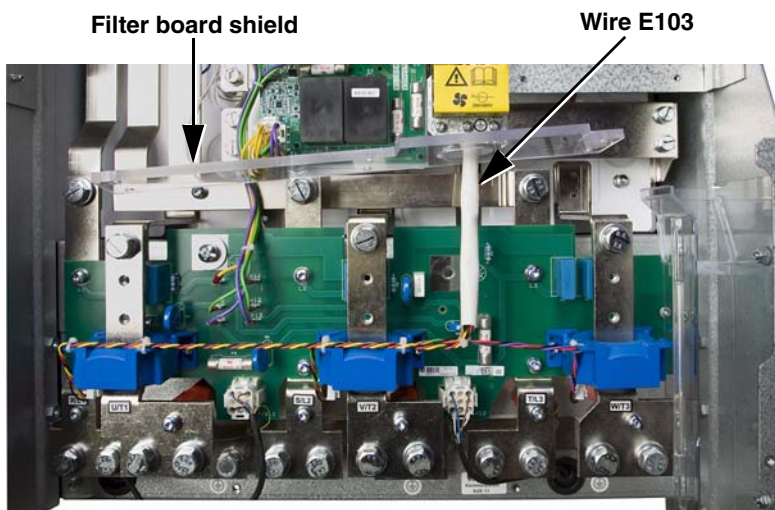
Figure 36: Filter Board Shield
