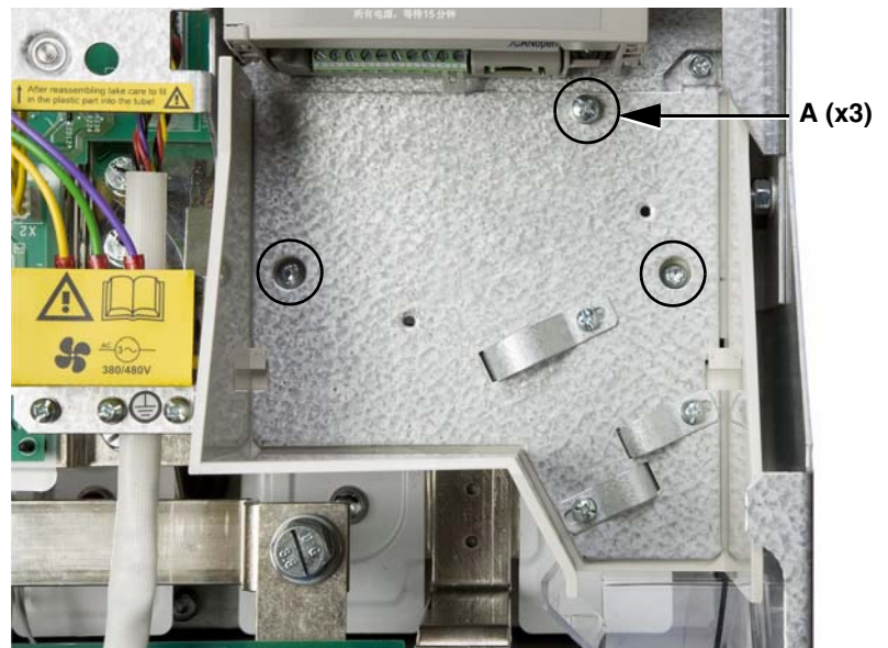
Figure 110: EMC Tray
