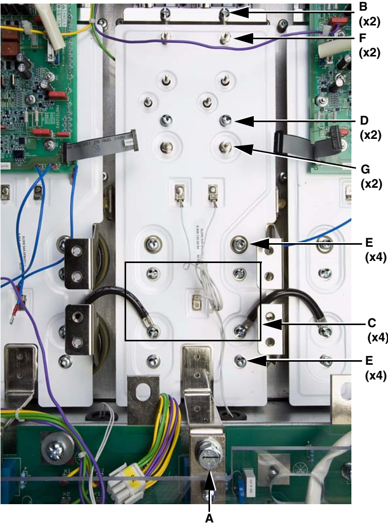
Figure 95: DC Bus Plate (Phase V Shown)
