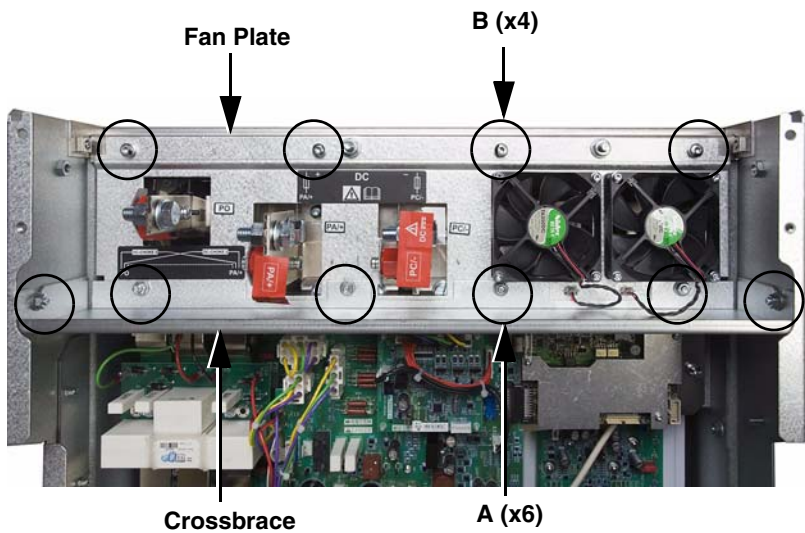
Figure 106: Fan Plate and Crossbrace
