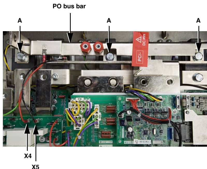
Figure 89: PO Bus Bar
