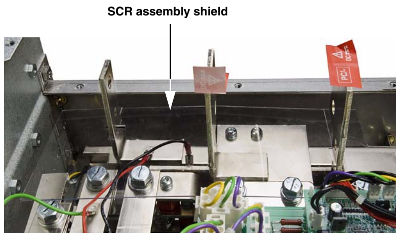
Figure 51: SCR Assembly Shield
