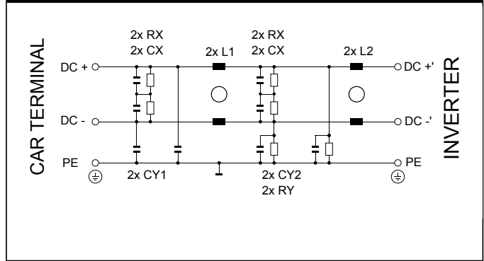
Typical electrical schematic FN223X (up to 500 VDC)
