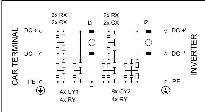
Typical electrical schematic FN222X and FN224X (up to 1000 VDC)
