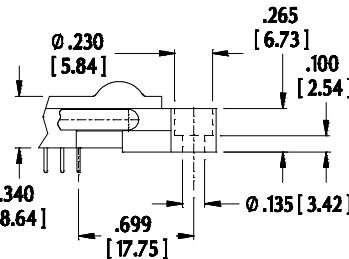
MOUNTING EAR DETAIL
