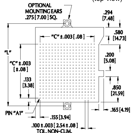
PCB FOOTPRINT (top view)
