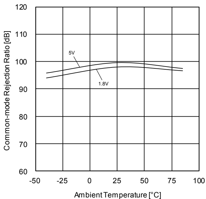
Figure 46. Common-mode Rejection Ratio vs Ambient Temperature
