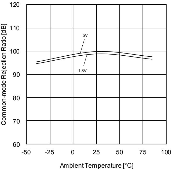
Figure 68. Common-mode Rejection Ratio vs Ambient Temperature
