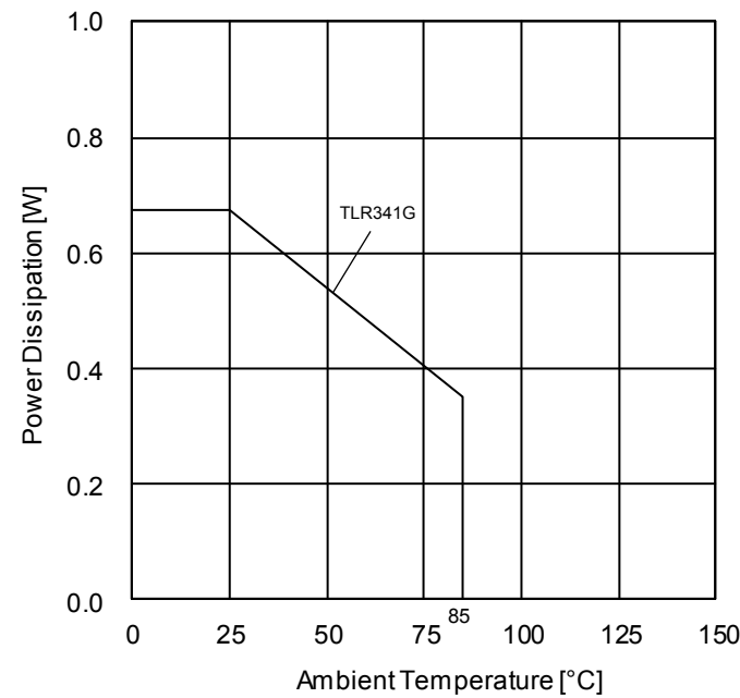
Figure 1. Power Dissipation vs Ambient Temperature (Derating Curve)
