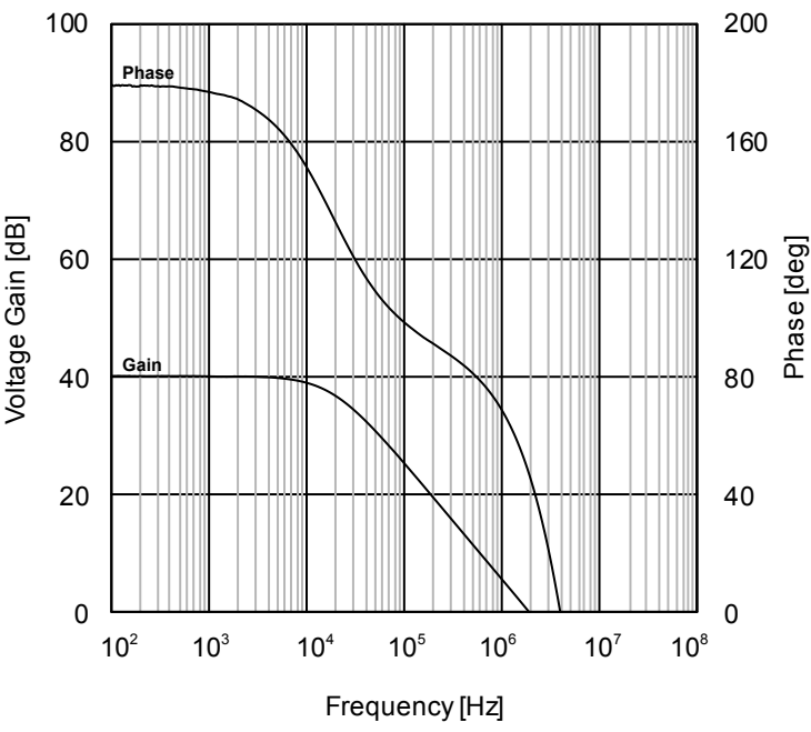
Figure 50. Voltage Gain, Phase vs Frequency (V DD =1.8V, T A =25°C)
