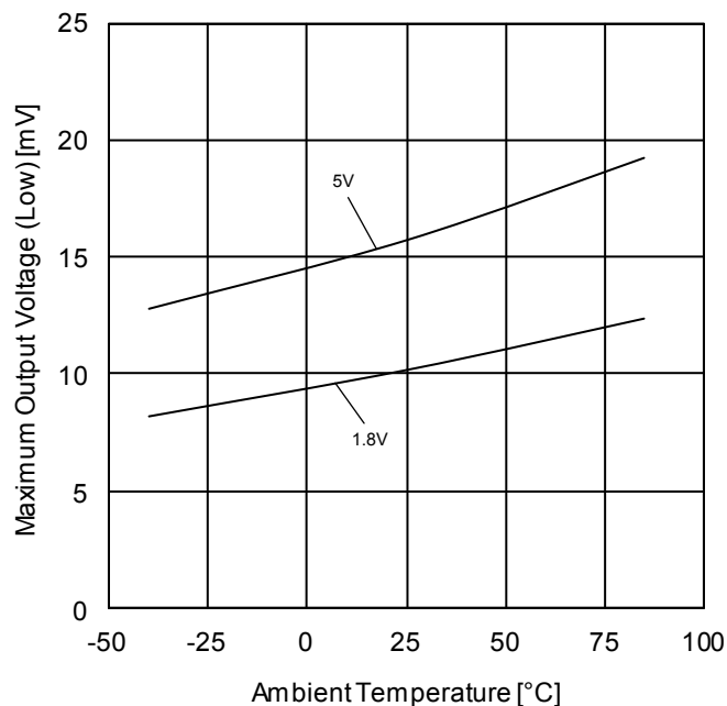
Figure 35. Maximum Output Voltage (Low) vs Ambient Temperature ( R_L=2k\Omega )
