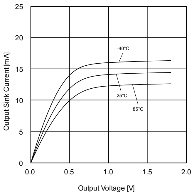
Figure 38. Output Sink Current vs Output Voltage ( V_{DD}=1.8V )
