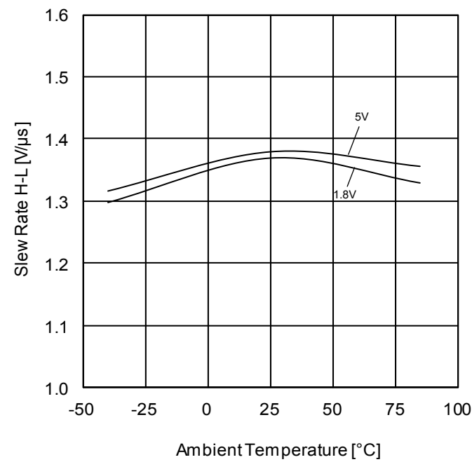
Figure 49. Slew Rate H-L vs Ambient Temperature
