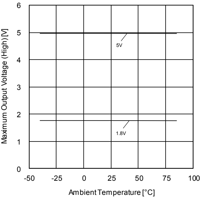
Figure 55. Maximum Output Voltage High vs Ambient Temperature ( R_L=2k\Omega )
