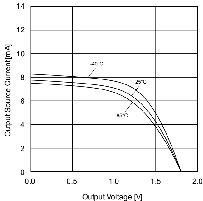
Figure 36. Output Source Current vs Output Voltage ( V_{DD}=1.8V )
