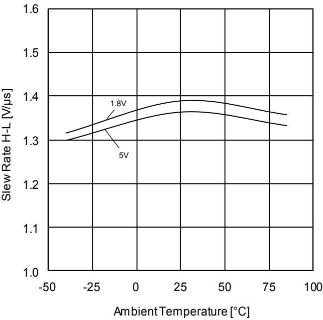
Figure 71. Slew Rate H-L vs Ambient Temperature
