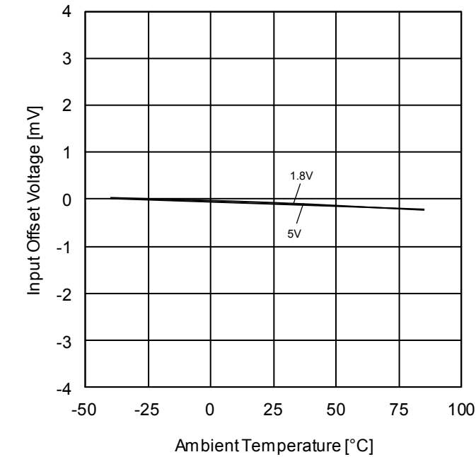
Figure 41. Input Offset Voltage vs Ambient Temperature
