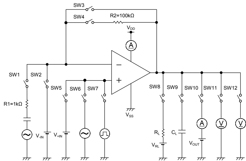
Figure 74. Test Circuit 2 (Each Op-Amp)
