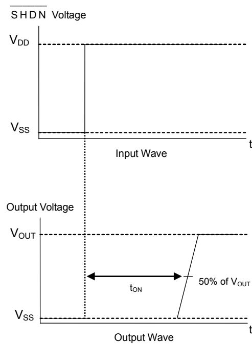
Figure 76. Turn On Time Input and Output Wave
