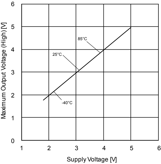
Figure 54. Maximum Output Voltage High vs Supply Voltage ( R_L=2k\Omega )
