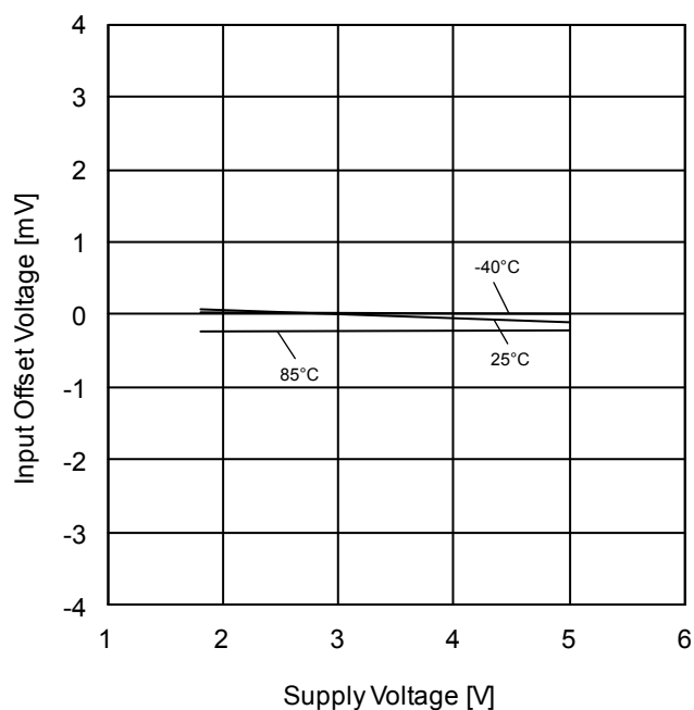
Figure 40. Input Offset Voltage vs Supply Voltage
