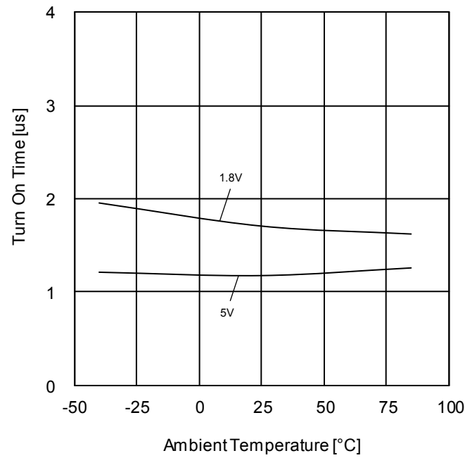
Figure 26. Turn On Time vs Ambient Temperature
