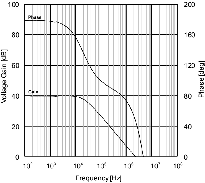
Figure 72. Voltage Gain, Phase vs Frequency (V DD =1.8V, T A =25°C)
