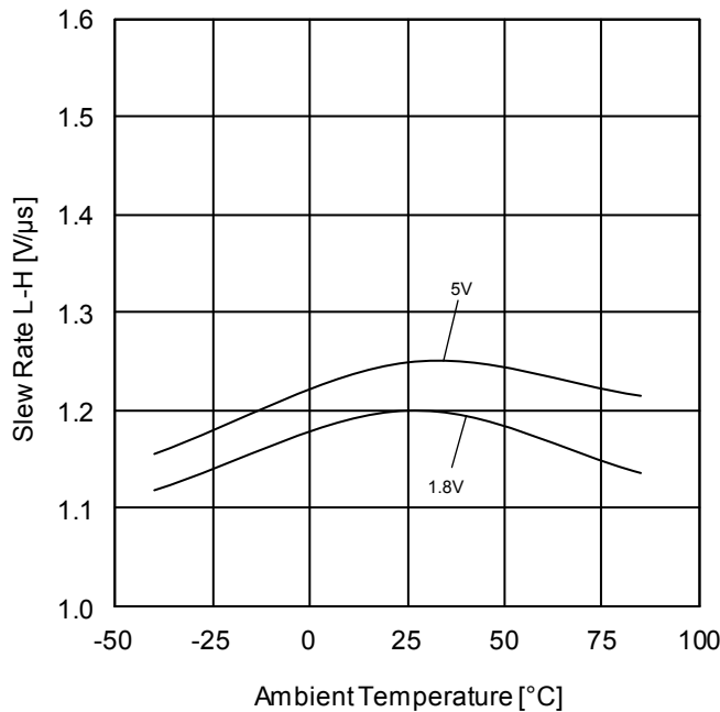
Figure 70. Slew Rate L-H vs Ambient Temperature
