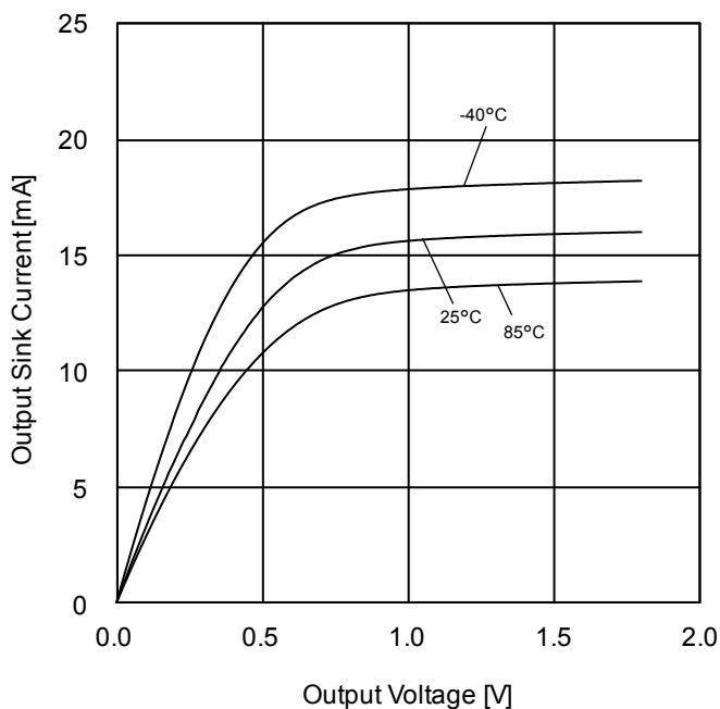
Figure 60. Output Sink Current vs Output Voltage ( V_{DD}=1.8V )
