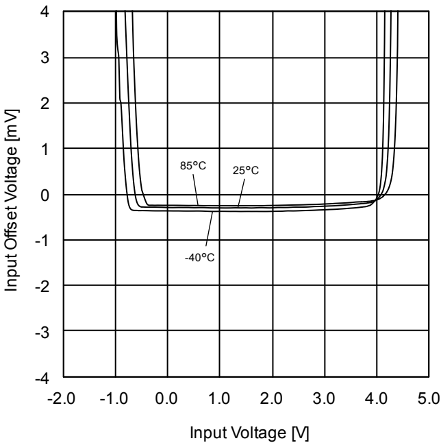
Figure 64. Input Offset Voltage vs Input Voltage ( V_{DD}=5V )
