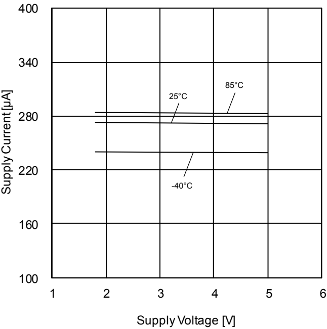
Figure 52. Supply Current vs Supply Voltage
