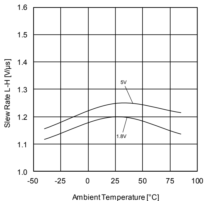
Figure 48. Slew Rate L-H vs Ambient Temperature
