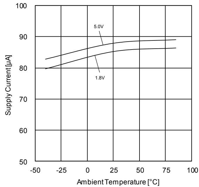
Figure 3. Supply Current vs Ambient Temperature
