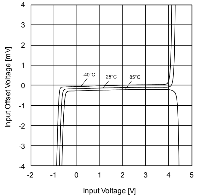
Figure 42. Input Offset Voltage vs Input Voltage (V DD =5V)
