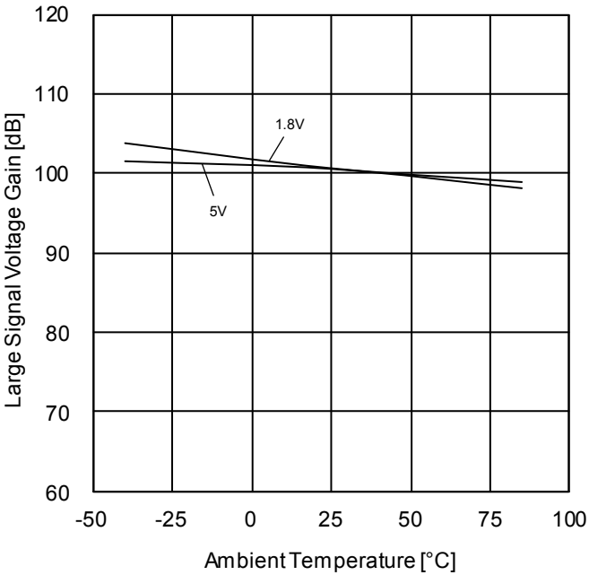
Figure 66. Large Signal Voltage Gain vs Ambient Temperature ( R_L=2k\Omega )
