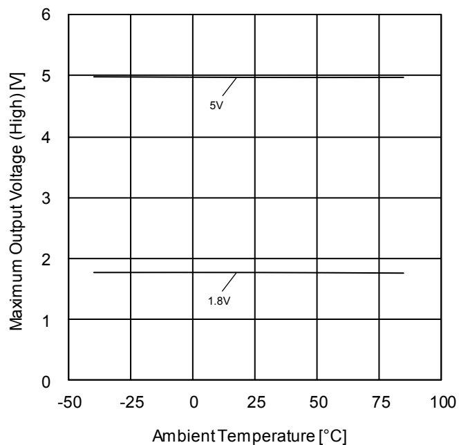
Figure 33. Maximum Output Voltage High vs Ambient Temperature ( R_L=2k\Omega )
