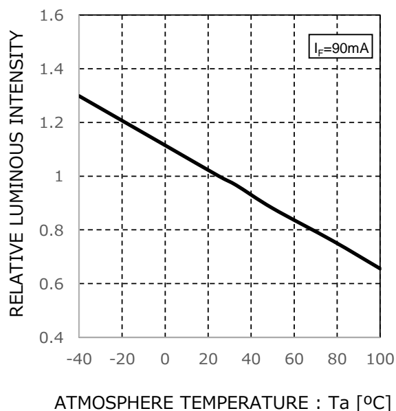
Fig.2 Luminous Intensity - Atmosphere Temperature
