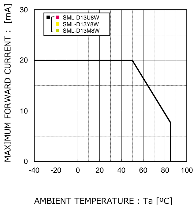
Fig.4 Derating
