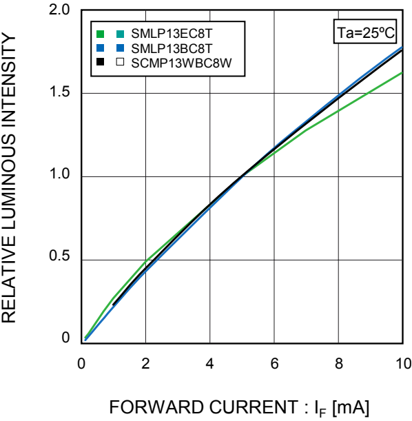
Fig.4 Luminous Intensity - Forward Current
