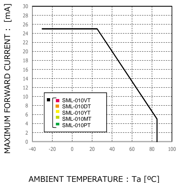
Fig.4 Derating
