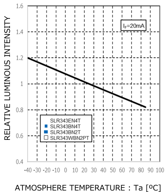
Fig.2 Luminous Intensity - Atmosphere Temperature
