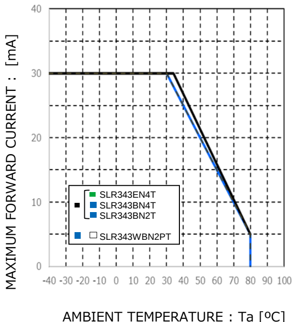
Fig.4 Derating
