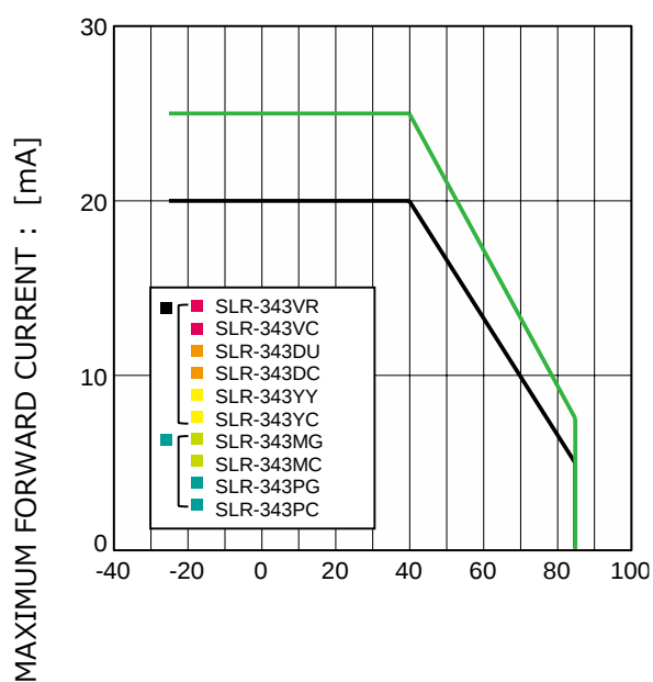
Fig.4 Derating
