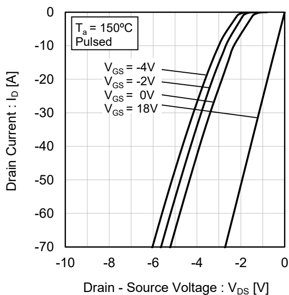
Fig.9 T_j = 150^\circ\text{C} 3rd Quadrant Characteristics
