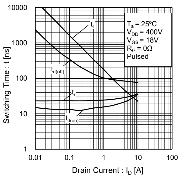
Fig.17 Switching Characteristics
