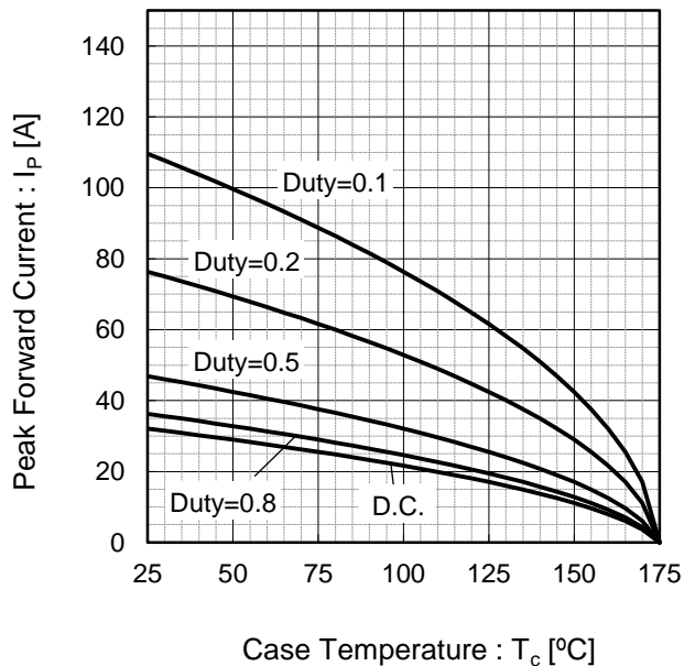
Fig.7*5 Maximum peak forward current derating curve I_P - T_c (Per Leg)
