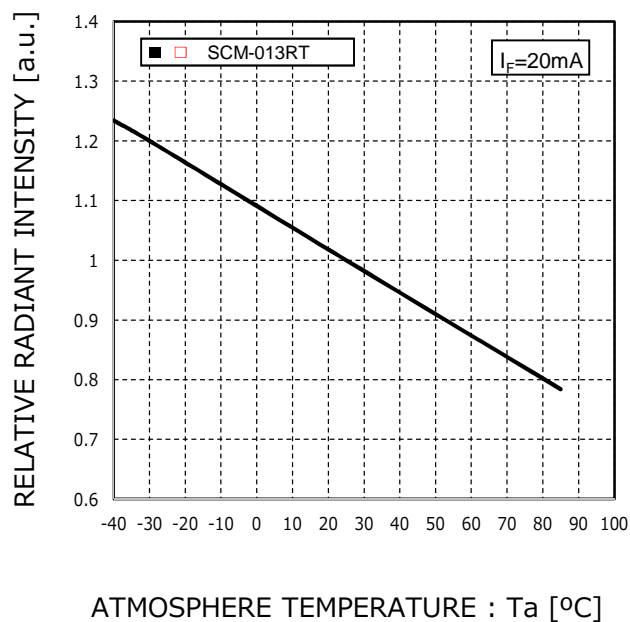
Fig.2 RADIANT Intensity - Atmosphere Temperature
