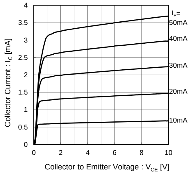
Fig.9 Output Characteristics
