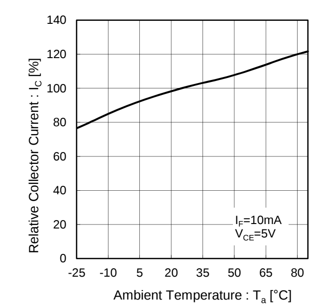
Fig.7 Relative Output vs. Ambient Temperature
