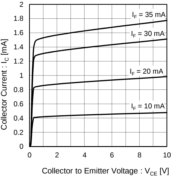
Fig.10 Output Characteristics
