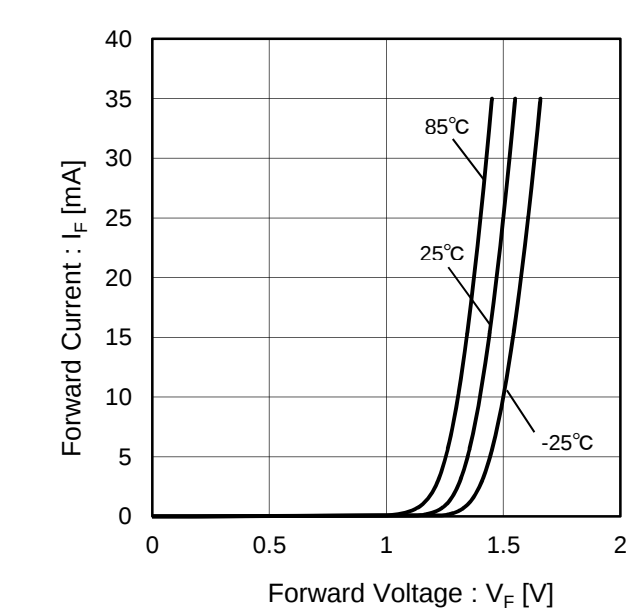
Fig.5 Forward Current vs. Forward Voltage
